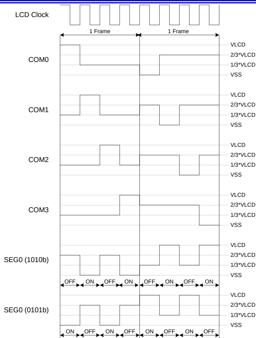
LCD 驱动波形, 1/4 duty, 1/3 bias
