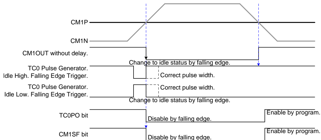
Stop TC0 pulse output @falling edge trigger, without delay.
