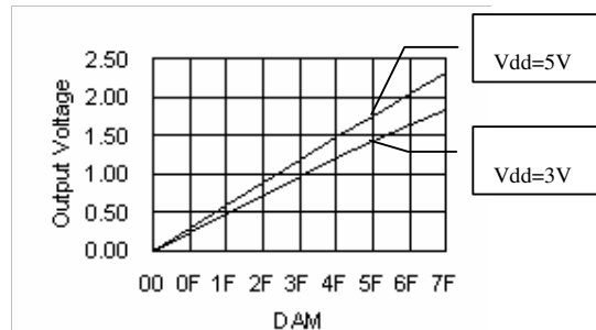
DAC Output Voltage in V_{dd}=5V and 3V
