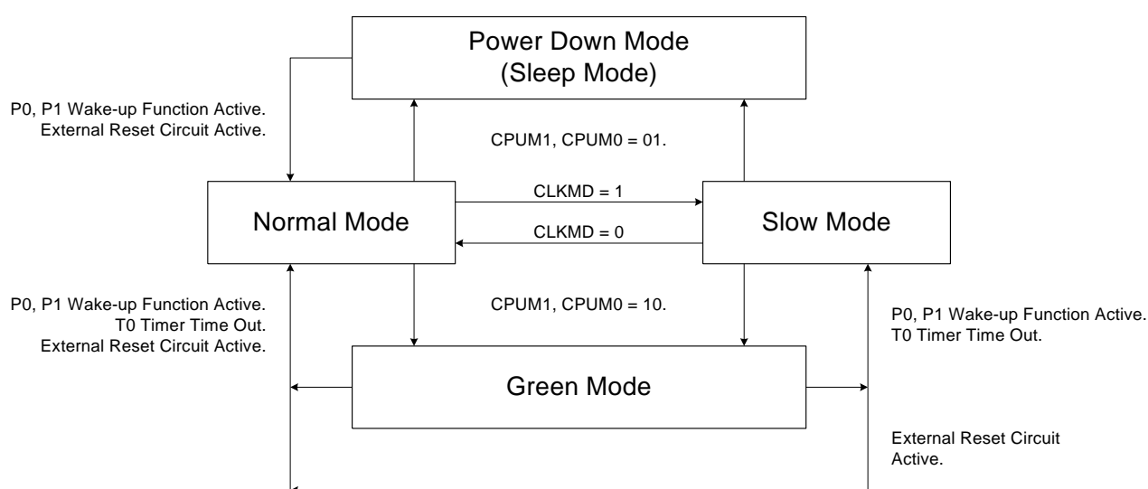
System Mode Switching Diagram
