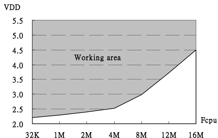
Working Voltage vs. Frequency (Noise Filter Disable、25°C)
