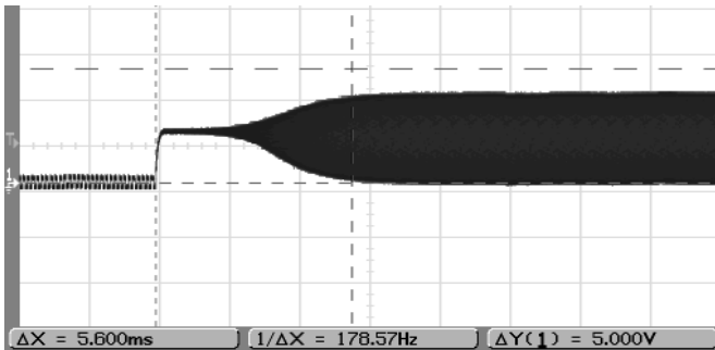
32768Hz Crystal
