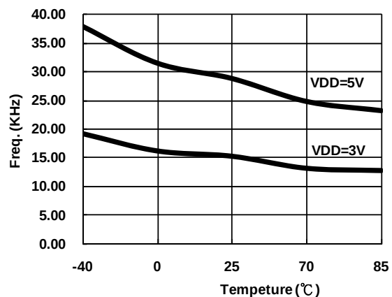
Internal Low RC Oscillator (KHz)
