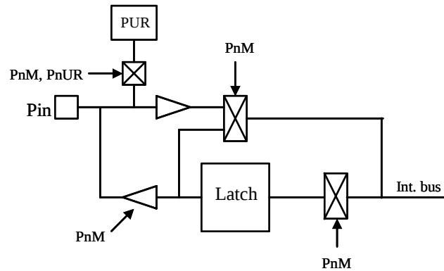
Port1,Port4,Port5 structure
