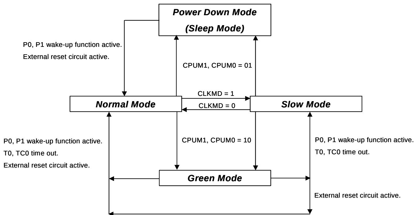
Figure 7-5. SN8P1800 System Mode Block Diagram
