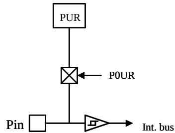
Port0.0~P0.2 structure
