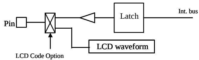
Port2 structure
